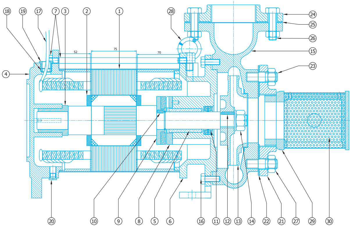
Cross sectional view of "Mahendra" Horizontal openwell submersible monobloc (ECM) pumpsets
